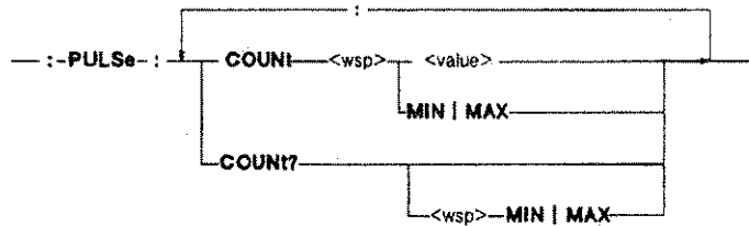
Figure 7-3. :PULSe:COUNT Syntax Diagram
