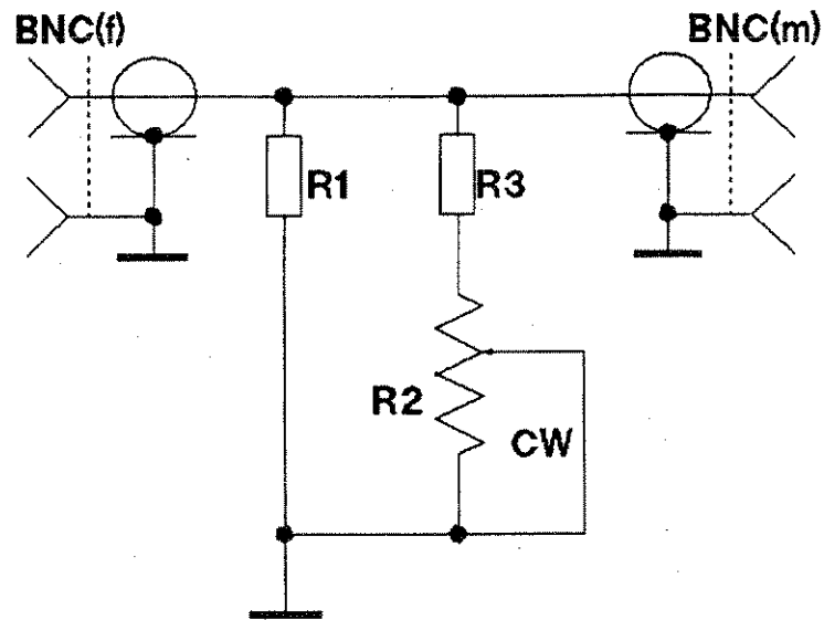
Figure C-1. 50, 0.1%, 10W Feedthrough Termination
