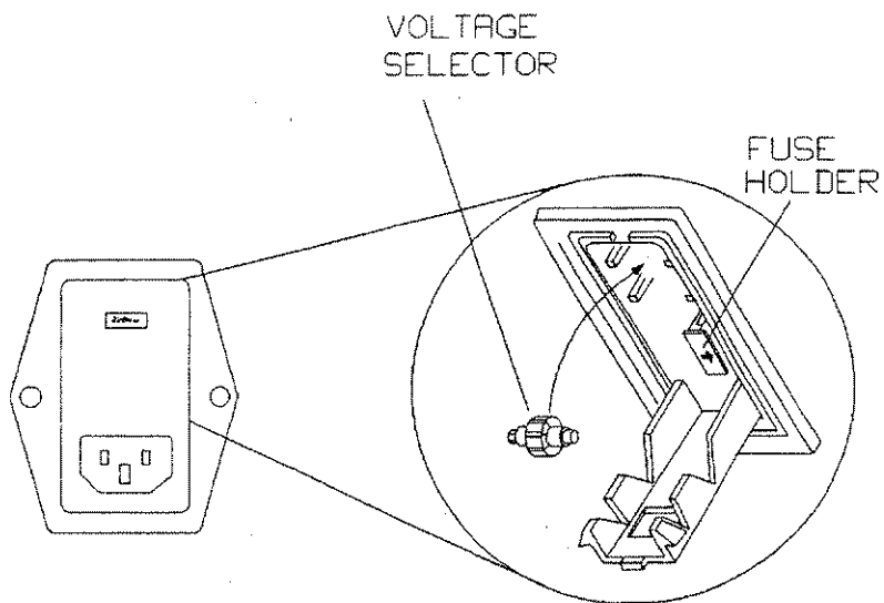
Figure 0-1. Line Voltage Switch Assembly
