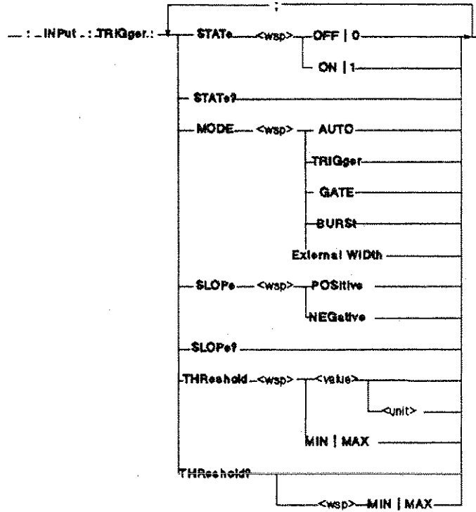
Figure 7-1. :INPut:TRIGger Syntax Diagram
