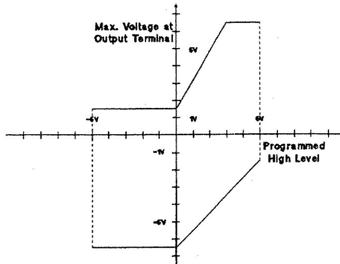
Figure 5-1. Output Voltage Window
