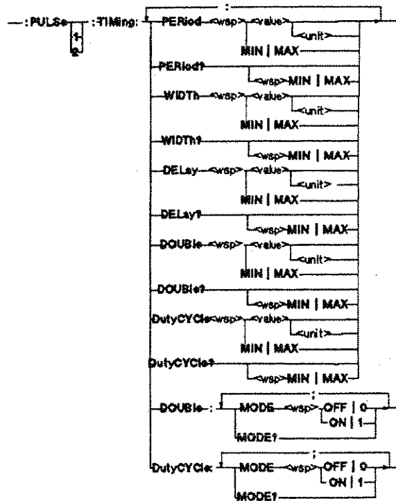
Figure 7-6. :PULSe:TIMing Syntax Diagram
