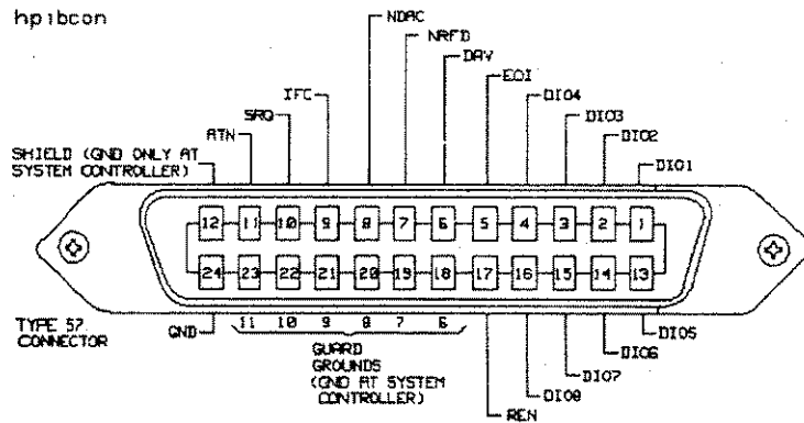
Figure A-3. HP-IB Connector
